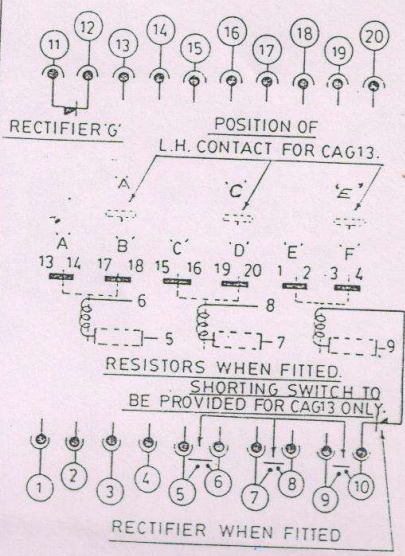
TERMINAL POSITIONS - DRAWOUT CASES VIEWED FROM FRONT.
